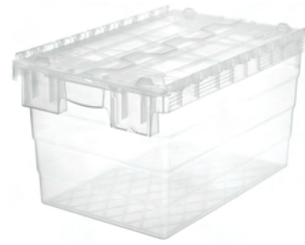
HP-6435-MK SF En/W Boy/L Yüksek/H Dış / Ext 400 x 600 x 360 mm İç / Int 365 x 545 x 347 mm Litresi / Liters : 70,00 Lt.
