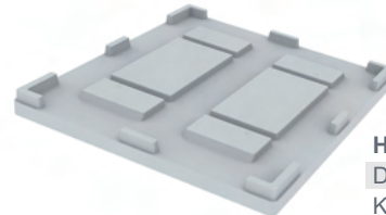
K-550-T En/W Boy/L Yüksek/H Hacim Dynamic Static Dış / Ext 800 x 1200 x 925 mm Volume Capacity Capacity İç / Int 732 x 1106 x 617 mm 500 Lt 400 Kg 2500 Kg Kapalı / Closed Ağırlık / Weight 22,50 kg
